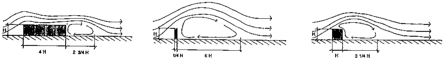
Fig 3/66 Influence of building depth
