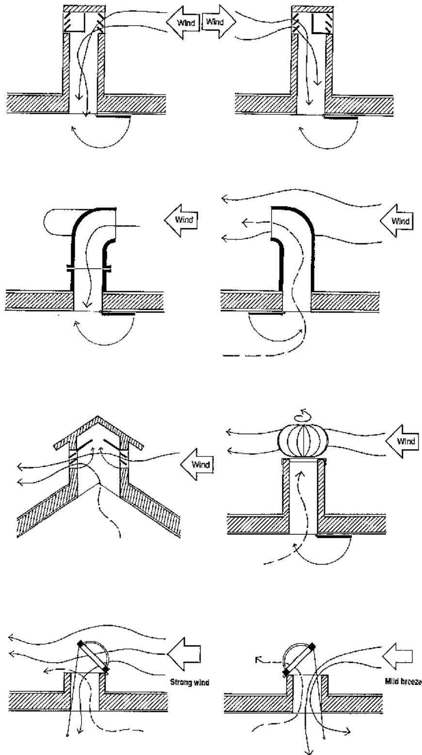
Fig 3/78 Examples of devices using external winds
