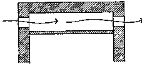
Fig 3/111 Ventilated double roof with light ceiling
