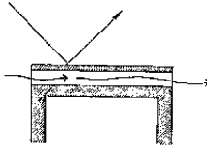
Fig 3/110 Ventilated double roof with heavy ceiling
