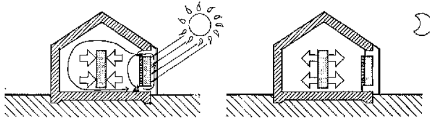
Fig 3/168 Solar wall as an air heating device with internal storage mass
