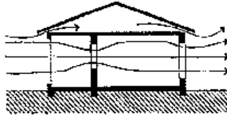
Fig 3/140 Large openings and screened-in porches.
