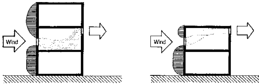
Fig 3/74 Deflection in the vertical direction
