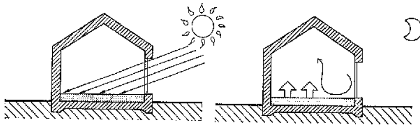
Fig 3/164 The floor as collector and heat storage mass
