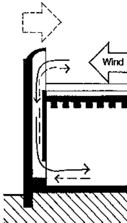
Fig 3/114 Unidirectional roof windcatcher
