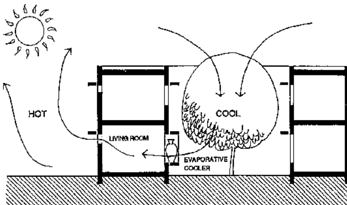
Fig 3/117 Cooling system of a courtyard house
