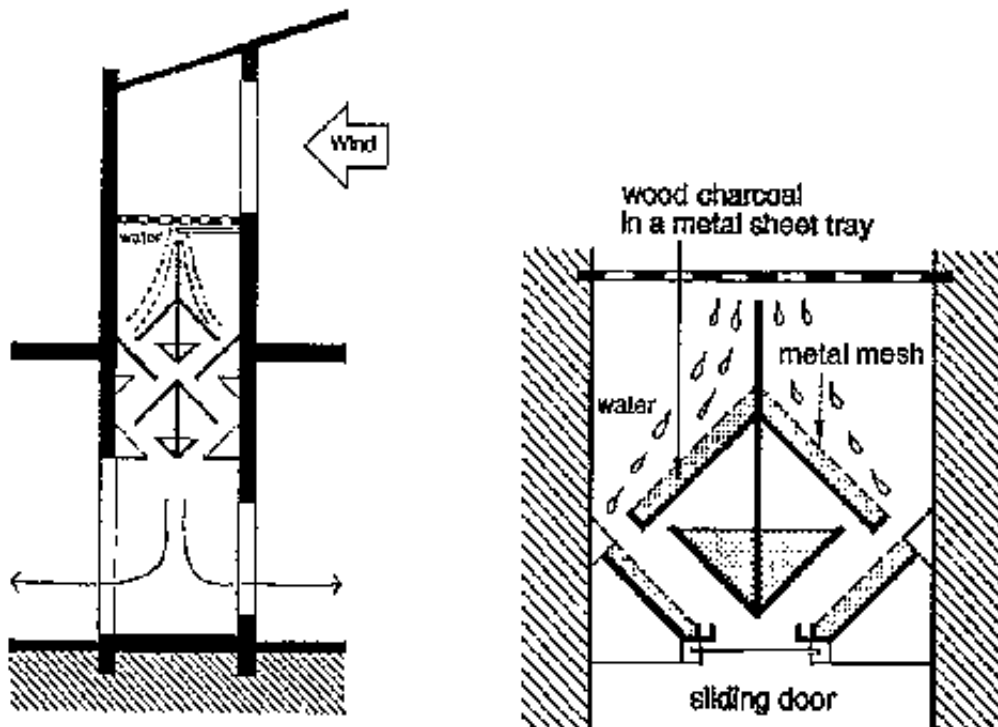
Fig 3/119 Evaporative cooler combined with a wind tower [-122 ]
