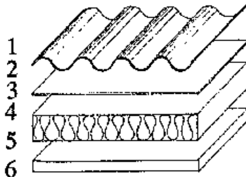
Fig 3/144 Suitable double leaf construction
