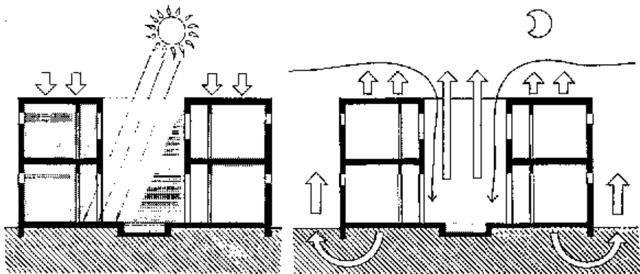
Fig 3/100 Courtyard house with covered galleries and an internal pool for evaporation, day and night situation
