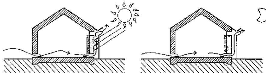
Fig 3/169 Solar wall as cooling device
