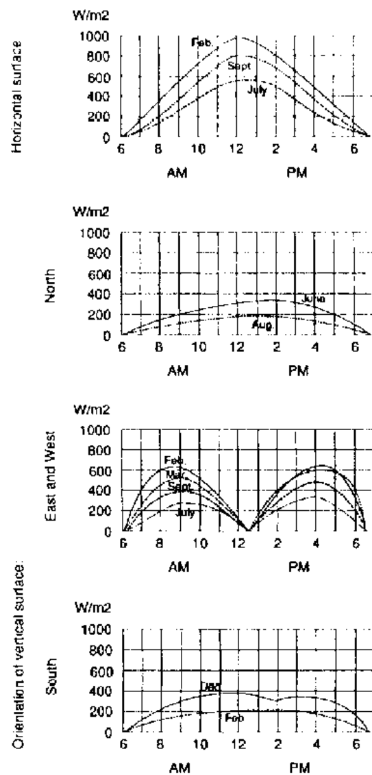
Fig 3/17 Analysis of the solar radiation intensity in Nairobi [ 8 ]
